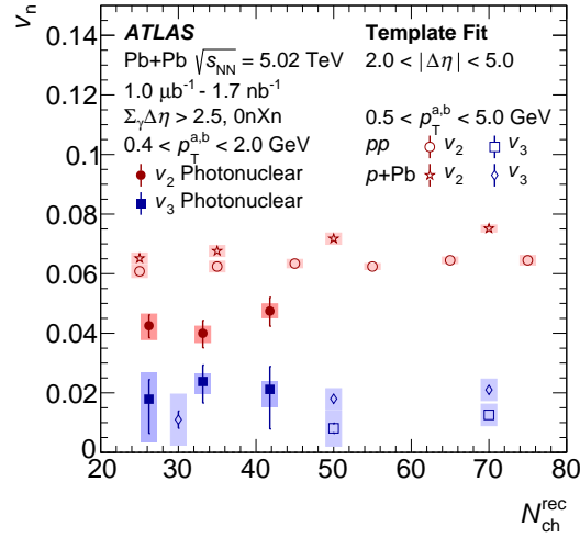
Figure 1.8: The v_n measurement results in UPC Pb+Pb, pp at 13 TeV, and p -Pb at 5.03 TeV as a function of multiplicity of the reconstructed charged particles tracks. Figure from [34].
