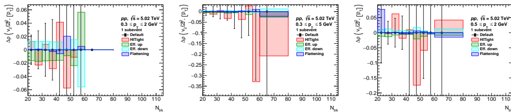
Figure D.17: Difference of 1-sub-event \rho(v_2\{2\}^2, [p_T]) in pp 5.02 TeV between different systematic uncertainties sources and baseline measurement \Delta_{\text{source}} in various p_T ranges, statistical uncertainty for baseline measurement is shown as a black line.
