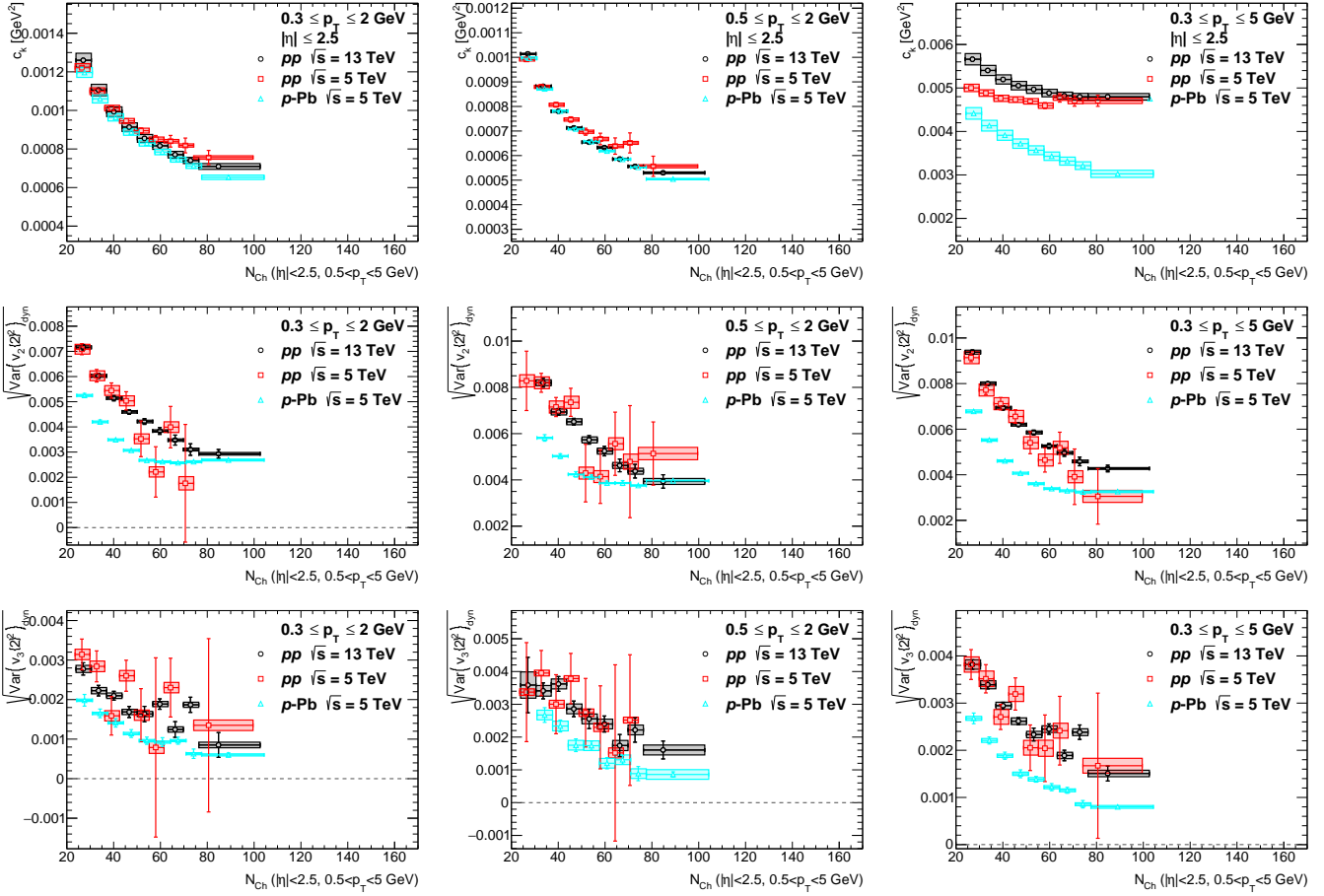
Figure 6.14: The comparison of c_k and \text{Var}(v_n\{2\}^2)_{\text{dyn}} between different collision systems and energy.
