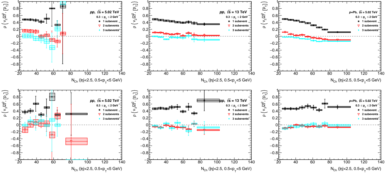
Figure 6.10: Comparison of \rho(v_n\{2\}^2, [p_T]) in various sub-events for each p_T range, from left to right columns for pp collisions at 5.02 and 13 TeV, and for p -Pb at 5.02 TeV respectively. The top rows is for n = 2 , and the bottom row is for n = 3 .
