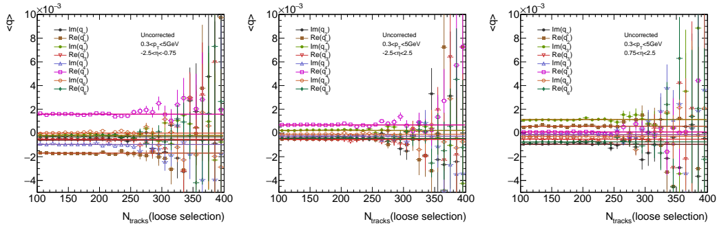
Figure C.1: Comparison of \langle q_n \rangle(N_{\text{tracks}}) for three sub-events, A - left, all - center, and C on the right. Fitted constant functions are the mean values of q_n -biases used in the analysis.
