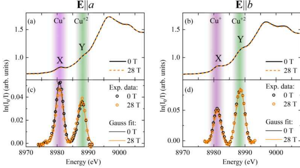
Figure 3.9: Pulsed-field XANES results obtained for YBCO with the incident beam polarized along a and b -axis, at 2 K. (a,b) Cu K -edge spectra collected in the absence of magnetic field and at 28 T are marked with a black solid and orange dashed line, respectively. According to literature, both features can be assigned to a distinct copper valence states ( 1^+ or 2^+ ) [33]. (c,d) Background subtracted spectra at 0 T and 28 T. The solid lines are Gaussian functions fitted to the experimental data.
