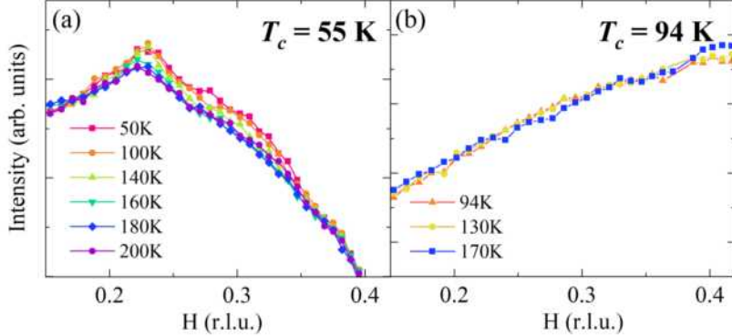
Figure 2.7: RXS spectra across the CDW wave vector measured at selected temperatures, in two Hg1201 samples with (a) T_c = 55 K ( p = 0.064 ) and (b) T_c = 94 K ( p = 0.126 ).
