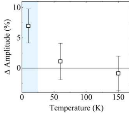
Figure 3.11: Temperature dependence of the relative change in the peak X amplitude between field range where the 3D order is absent and 28 T ( \Delta Amplitude). Blue shaded area indicates the temperature range, where 3D CDW order appears. Errors are obtained from the fitting procedure. The error of \Delta Amplitude is determined using propagation of uncertainty method.
