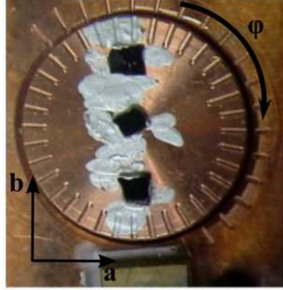
Figure 2.3: Single crystals of Hg1201 mounted on the cold-finger of a liquid He cryostat, inside the vacuum chamber operating in the pressure range of 10^{-9} mbar. The samples were glued using a silver paint. Typical sample volume was about 1 - 2 \text{ mm}^3 . The sample surface corresponds to the crystallographic ab plane. The \varphi angle is usually used to adjust the angular position and by that precisely orient the crystals. Only one sample was measured at a time, but inserting three crystals saved the time needed to achieve UHV.
