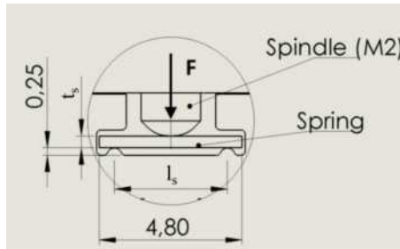
Figure 6.4: Application of the force in the spring-driven 'Solaris' uniaxial pressure cell. F indicates the direction of an applied force. The screw presses on the spring exactly in the middle of l_s . In case of resistivity measurements presented in this section t_s = 0.51 mm and l_s = 3.8 mm.
