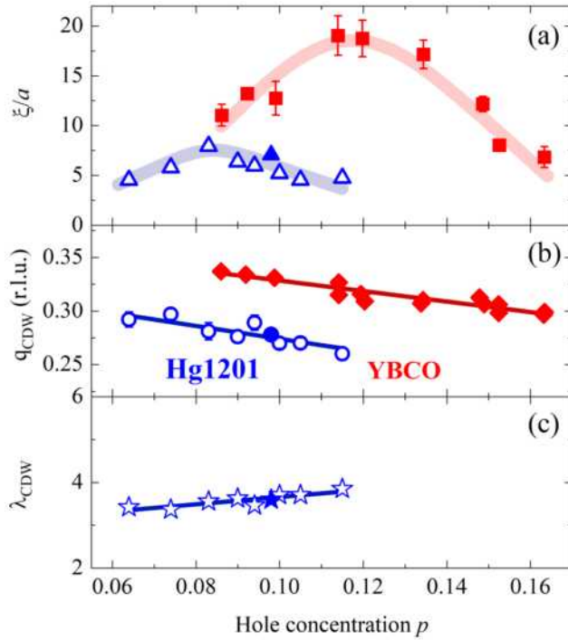
Figure 2.6: Parameters characterizing the CDW order in Hg1201 obtained from Gaussian fits presented in Fig. 2.5 (blue symbols) compared with corresponding parameters for YBCO (red symbols) from [8]. Filled blue symbols indicate RXS and XRD data for Hg1201 from Tabis et al. [1]. (a) The correlation length \xi/a , (b) wave vector q_{CDW} , and (c) wave length \lambda_{CDW} of the CDW order are presented as a function of doping. Error bars corresponds to errors of the fitting parameters and are usually smaller than the symbols. The broad bands in (a) are guides-to-the-eye, the solid lines in (b) and (c) are linear fits.
