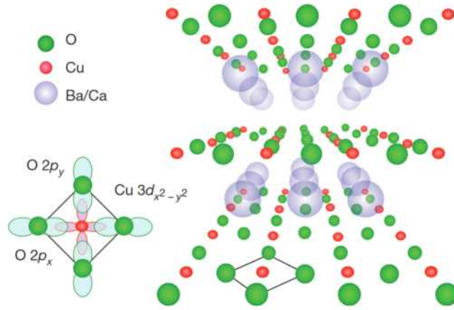
Figure 1.2: Schematic drawing of crystal structure of layered copper oxides [26]. CuO 2 planes are typically separated by insulating spacer layers (grey spheres). Within the planes, 3d_{x^2-y^2} holes on the Cu sites are hybridized with 2p_x and 2p_y oxygen orbitals.
