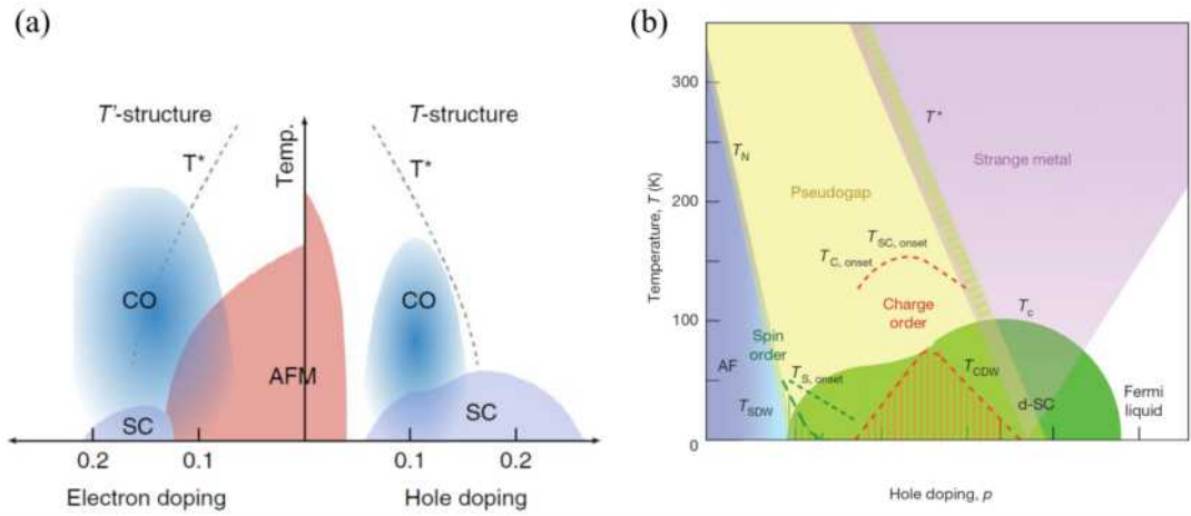
Figure 1.5: (a) Schematic, temperature-doping phase diagram of electron- and hole-doped cuprates [55]. Indicated are the antiferromagnetic (AFM) phase, superconducting (SC) phase and charge-ordered (CO) region. The pseudogap temperature T^* is indicated with dashed line. (b) One of many tentative phase diagram of hole-doped cuprates is shown to emphasise the complexity of these compounds, adapted from [26]. Different 'onset' temperatures (some of them compound specific) are associated with the appearance of precursors or fluctuations of certain orders: T_{s,onset} (dashed, green line) for spin order, T_{C,onset} for charge order and T_{SC,onset} for superconductivity (red, dashed line for both of them). According to the suggested phase diagram, fully developed spin density wave order appears below T_{SDW} , and the charge density wave order is considered long-range below T_{CDW} .
