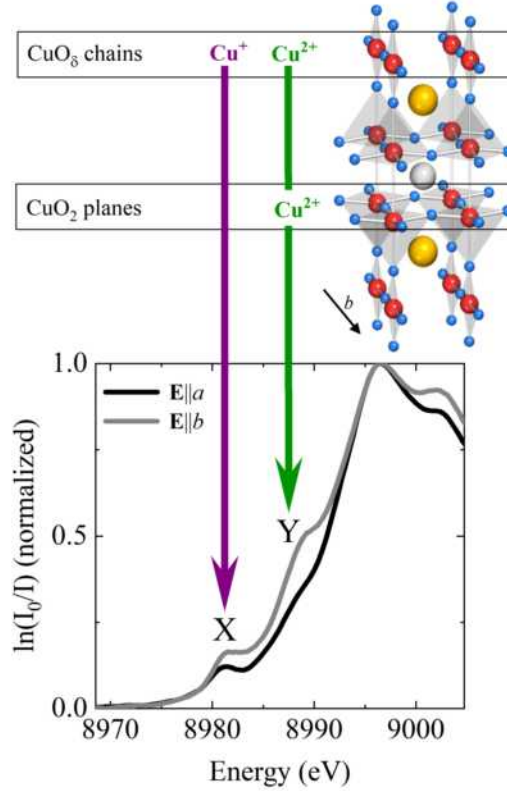
Figure 3.8: Elementary unit cell and XANES zero-field spectra of YBCO collected for two polarization directions. (top) YBCO is orthorhombic with two \text{CuO}_2 planes per primitive cell. The charge-carrier concentration in the \text{CuO}_2 planes is controlled through the variation of the interstitial O concentration within the \text{CuO}_\delta chains oriented along the b -axis, with various inter-chain ordering patterns. (Bottom) Cu K -edge absorption spectra of YBCO ( \delta = 0.55 ) collected at 2 K, with the incident beam polarization along a (black line) and along b (grey line). The two distinct peaks, X and Y , are observed at 8981 eV and 8989 eV. According to the literature data discussed in Section 3.3 they correspond to \text{Cu}^+ and \text{Cu}^{2+} sites, marked by the purple and green arrow, respectively.
