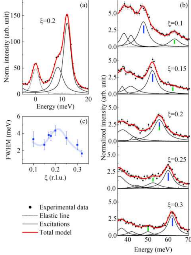
Figure 4.5: Experimental IXS spectra measured at 300 K for optimally doped sample ( x = 0.145 ) with a corresponding Lorentzian fits. (a) The low energy part of the spectrum consists of the elastic contribution marked by a dashed line and the acoustic phonons which are marked with solid lines. (b) Evolution of the high energy part of the IXS energy spectrum across the Brillouin zone for selected \xi values. (c) FWHM of the phonon mode marked by a blue bar in (b). The light blue line is a guide to eye. The error bars correspond to standard deviations of the fit coefficients, in (a) and (b) and represent the systematic errors associated with the experiment.
