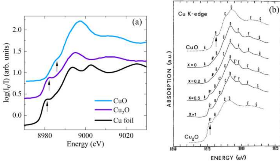
Figure 3.6: (a) Comparison between Cu K -edge XANES spectra of \text{Cu}^0 , \text{Cu}_2^1\text{O} and \text{Cu}^{2+}\text{O} . While the data for \text{Cu}^0 were obtained from our absorption measurements of a copper foil, the spectra of the two copper oxides are adapted from [32]. Black arrows indicate characteristic edge features discussed in the text. Figure (b) is adapted from [33] and shows XANES spectra for \text{YBa}_2\text{Cu}_3\text{O}_{7-x} (solid lines) at various doping levels compared with the reference copper oxides (dashed lines).
