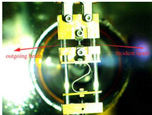
Figure 5.8: The spring-driven uniaxial pressure cell mounted inside the diffractometer chamber. Red arrow indicates the direction of the X-ray beam that scatters of the mounted sample.
